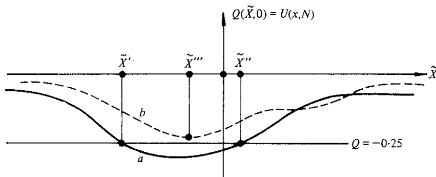
FIGURE 1. Current velocity distributions for: —, supercritical barrier; ---, subcritical barrier.
