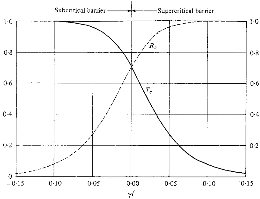
FIGURE 2. Reflexion ( R_c ) and transmission ( T_c ) coefficients for a parabolic barrier.
