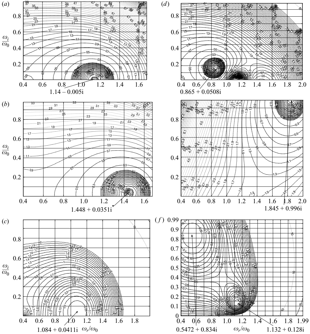
FIGURE 12. Isolines of \|G\|^2 for various wind and current conditions and \lambda=5 cm. (a)- u_* = 0.3 \text{ m s}^{-1} , no wind, exponential current, the eigenvalue is \omega/\omega_0 = 1.14 - 0.005i , (b) u_* = 0.3 \text{ m s}^{-1} , numeric wind profile, constant current, the eigenvalue is \omega/\omega_0 = 1.448 + 0.0351i , (c) u_* = 0.3 \text{ m s}^{-1} , numeric wind profile, exponential current, the eigenvalue is \omega/\omega_0 = 1.084 + 0.0411i , (d) u_* = 0.8 \text{ m s}^{-1} , no wind, exponential current, the eigenvalue is \omega/\omega_0 = 0.865 + 0.0508i , (e)- u_* = 0.8 \text{ m s}^{-1} , numeric wind profile, constant current, the eigenvalue is \omega/\omega_0 = 1.845 + 0.996i , (f)- u_* = 0.8 \text{ m s}^{-1} , numeric wind profile, exponential current, the eigenvalues are at \omega/\omega_0 = 0.5472 + 0.834i , \omega/\omega_0 = 1.132 + 0.128i . The numeric wind profile is according to the numerical solution of (2.23), and the exponential current is according to (2.21), with B = 0.5 .
