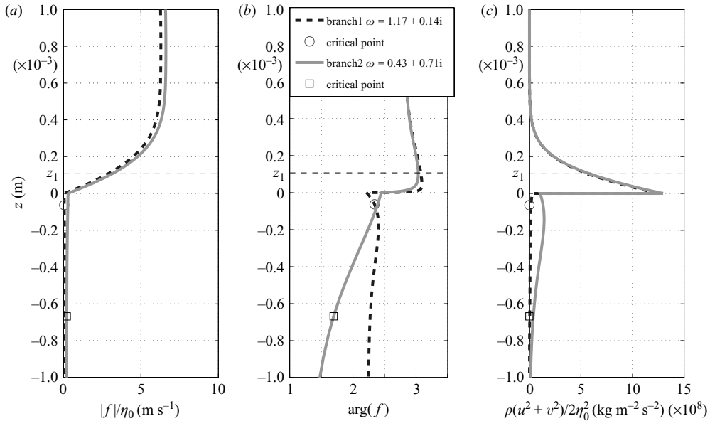
FIGURE 11. Comparison of the vertical structure of the eigenfunction and the kinetic energy density between the two modes for \lambda = 0.04 m, u_* = 0.7 m s -1 , temporal case, profile is according to (2.20)–(2.22). (a) absolute value of the eigenfunction, (b) argument of the eigenfunction, (c) kinetic energy density.
