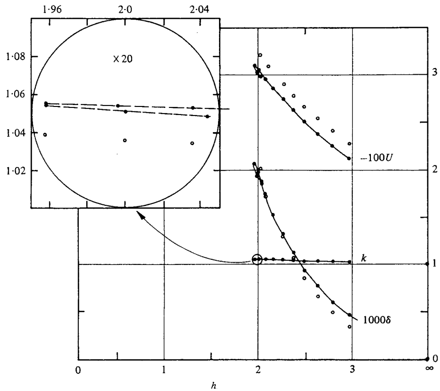
FIGURE 4. Theoretical variation of wavenumber k , set down \delta , and current U , with depth for deep water waves with \epsilon_{\infty}^2 = 0.7 , H_{\infty}/L_{\infty} = 0.118 . ●—●, Cokelet's method; ○ ○, linear theory.
