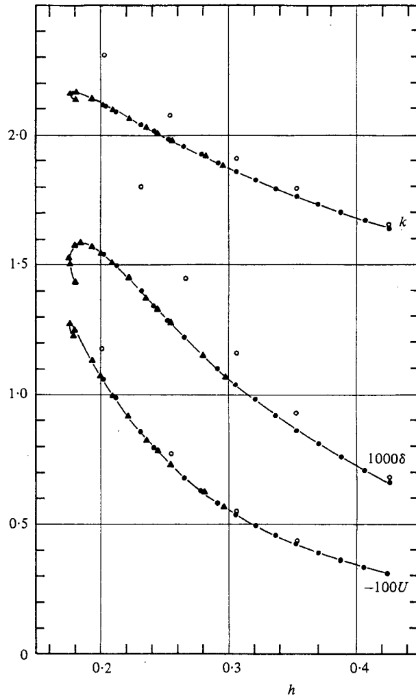
FIGURE 5. Theoretical variation of wavenumber k , set down \delta , and current U , with depth for deep water wave with \epsilon_\infty^2 = 0.01 , H_\infty/L_\infty = 0.013 . \bullet , Cokelet's method; \blacktriangle , TSW; \circ , linear theory.
