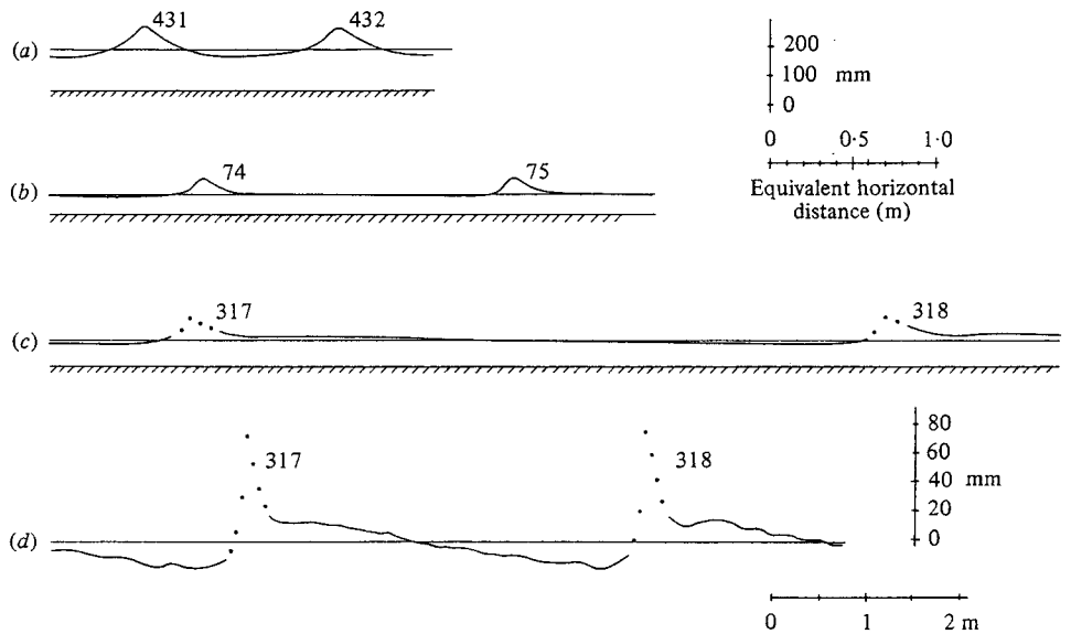
FIGURE 12. Profiles of waves in Hansen & Svendsen's (1979) experiments used for comparison in figures 9-11. They are all for the highest, or close to highest, waves. The profiles were measured as a function of time from a slowly-moving carriage. This has been converted to an equivalent horizontal distance, using the wave velocity. The vertical exaggeration is 7:4 for figures (a), (b) and (c), and is 15:1 for figure (d). (a) Test 101101: wave 430, D^* = 147.6 mm; wave 431, D^* = 146.4 mm. (b) Test A06113 (identical conditions to test A06103): wave 74, D^* = 71.0 mm; wave 75, D^* = 69.8 mm. (c) and (d) Test 031041; wave 317, D^* = 94.7 mm; wave 318, D^* = 92.7 mm. Individual data points are shown in the places where a smooth profile cannot easily be drawn.
