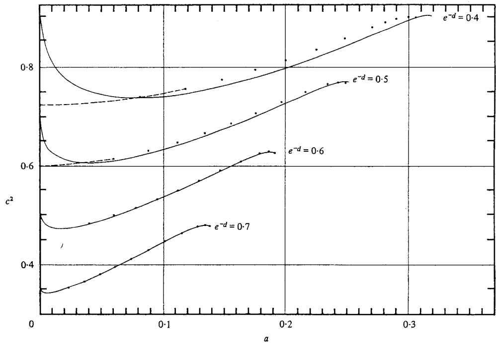
FIGURE 2. Comparison of phase velocity squared, c^2 , against amplitude, a , for waves on finite depth of water between Cokelet's (1977) solution (--- ● ● ●) and the train of solitary waves approximation (—).
